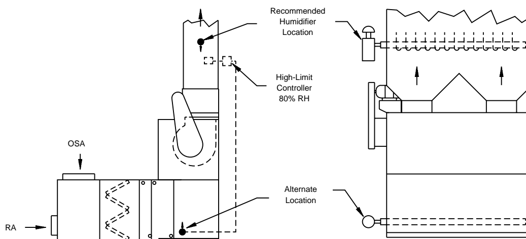
Figure 35-2. Vertical Discharge
