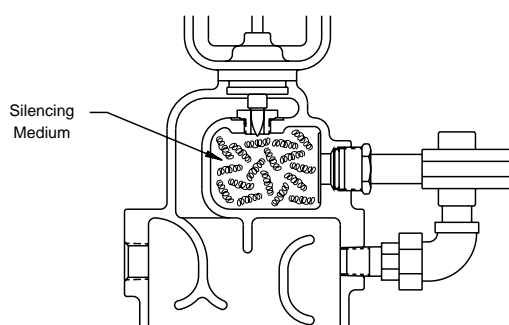
Figure 23-4. The noise of escaping steam is generated at the control valve. Muffling materials around the valve are necessary to minimize this noise.
