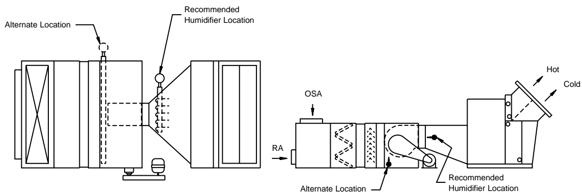
Figure 36-2. High pressure system
