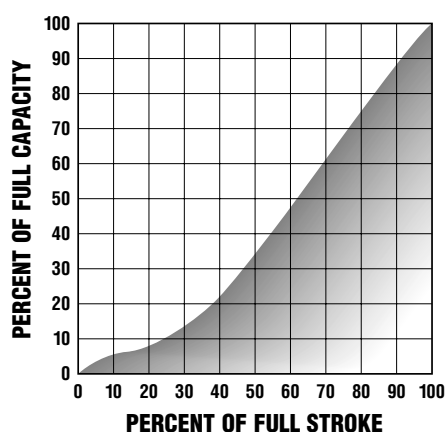
Chart 21-1. Desirable modified linear characteristic curve for valves used under modulating control. The modification of true linear characteristics provides more precise control when capacity requirements are very low and the valve is just cracked off the seat.
