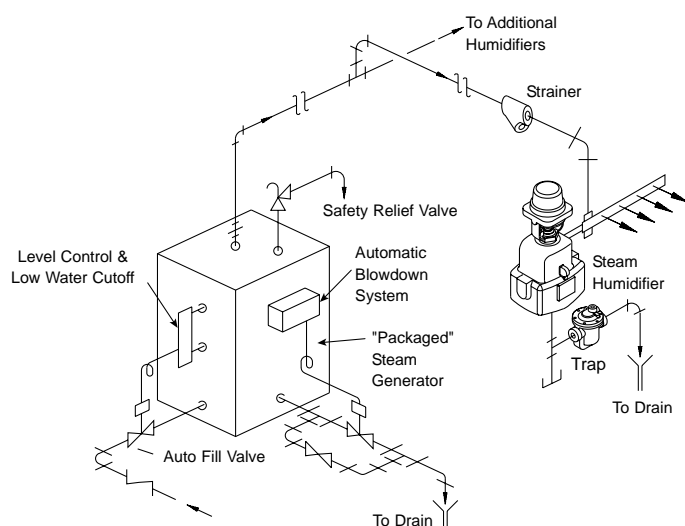
Figure 19-1. Typical Piping for Boiler-Humidifier Installation
