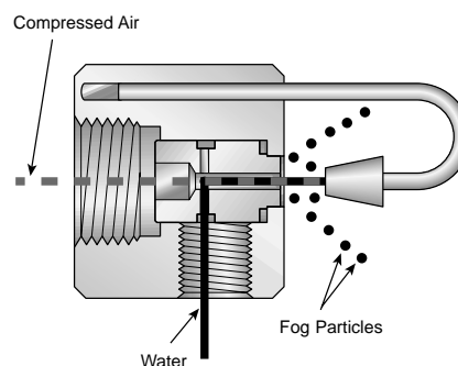
Figure 18-2. Fogger Head
