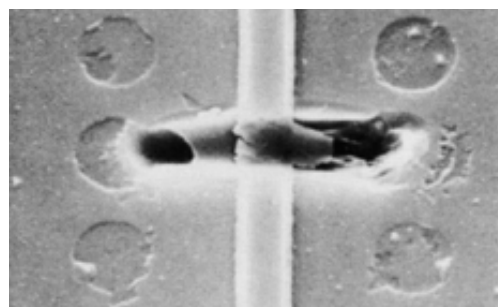
Integrated circuit damaged by ESD.
