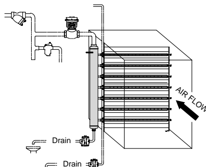
Figure 16-2. Panel Type
